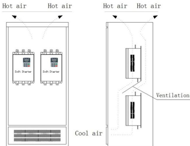
Figure3-2 Horizontal layout
