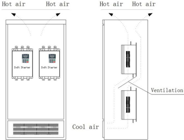
Figure3-2 Horizontal layout
