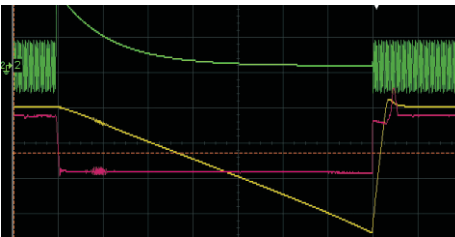
Speed tracing output frequency and current waveform
